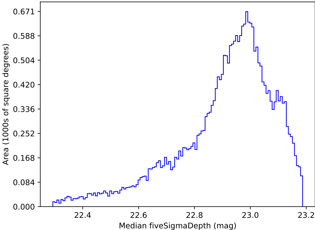
ddf_loaded_fl4_v3.4_10yrs All sky z band: Median fiveSigmaDepth
