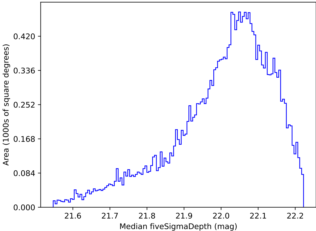
ddf_loaded_fl4_v3.4_10yrs All sky y band: Median fiveSigmaDepth
