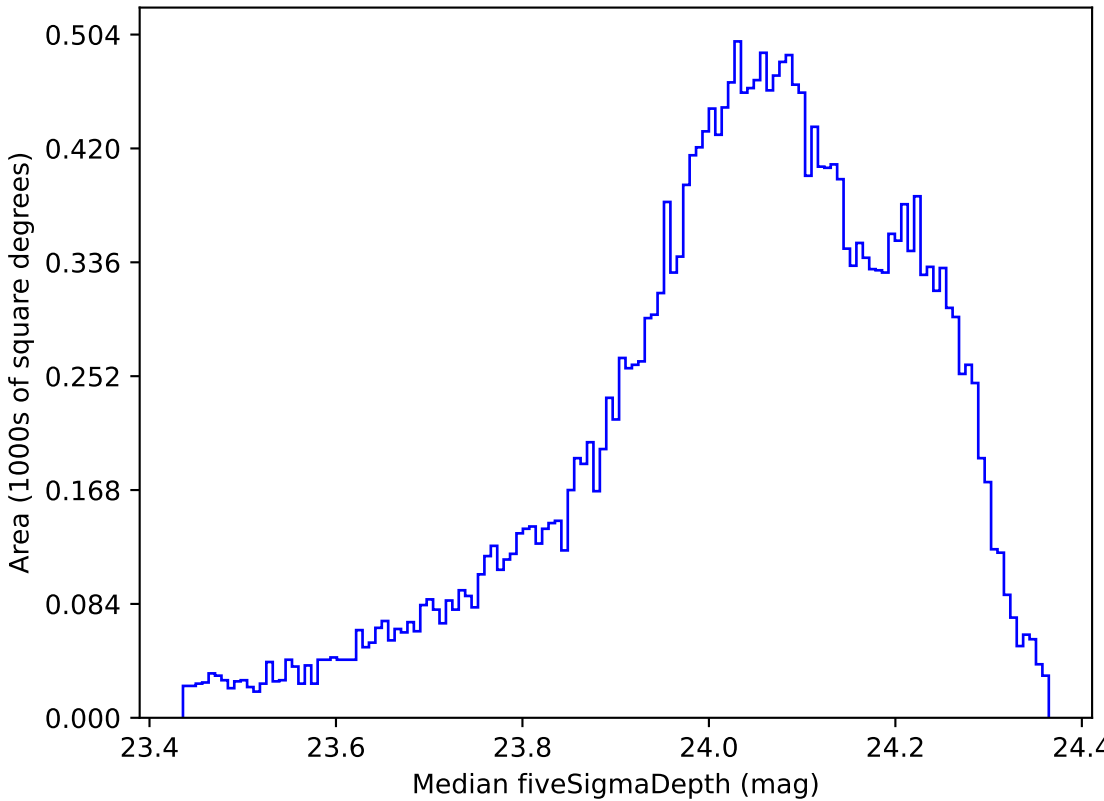
ddf_loaded_fl4_v3.4_10yrs All sky r band: Median fiveSigmaDepth
