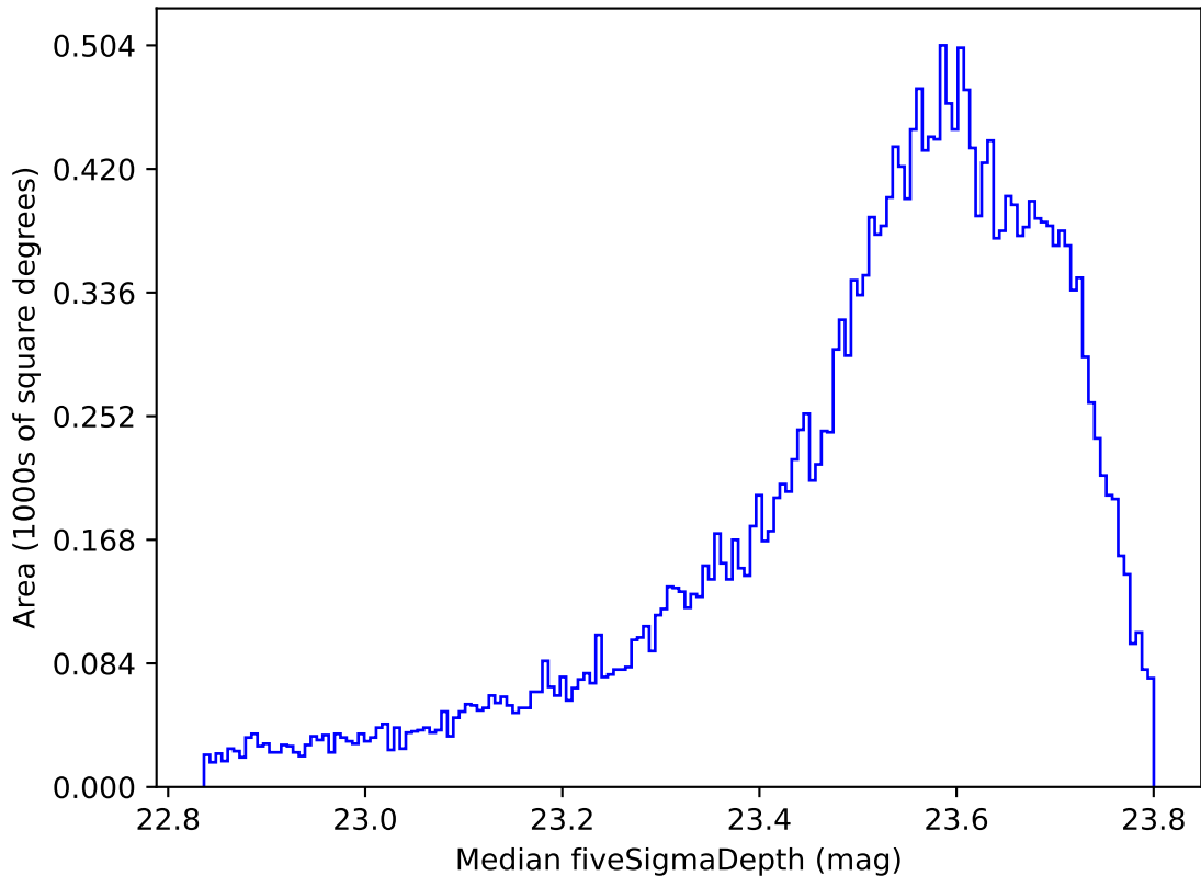
ddf_loaded_fl4_v3.4_10yrs All sky i band: Median fiveSigmaDepth
