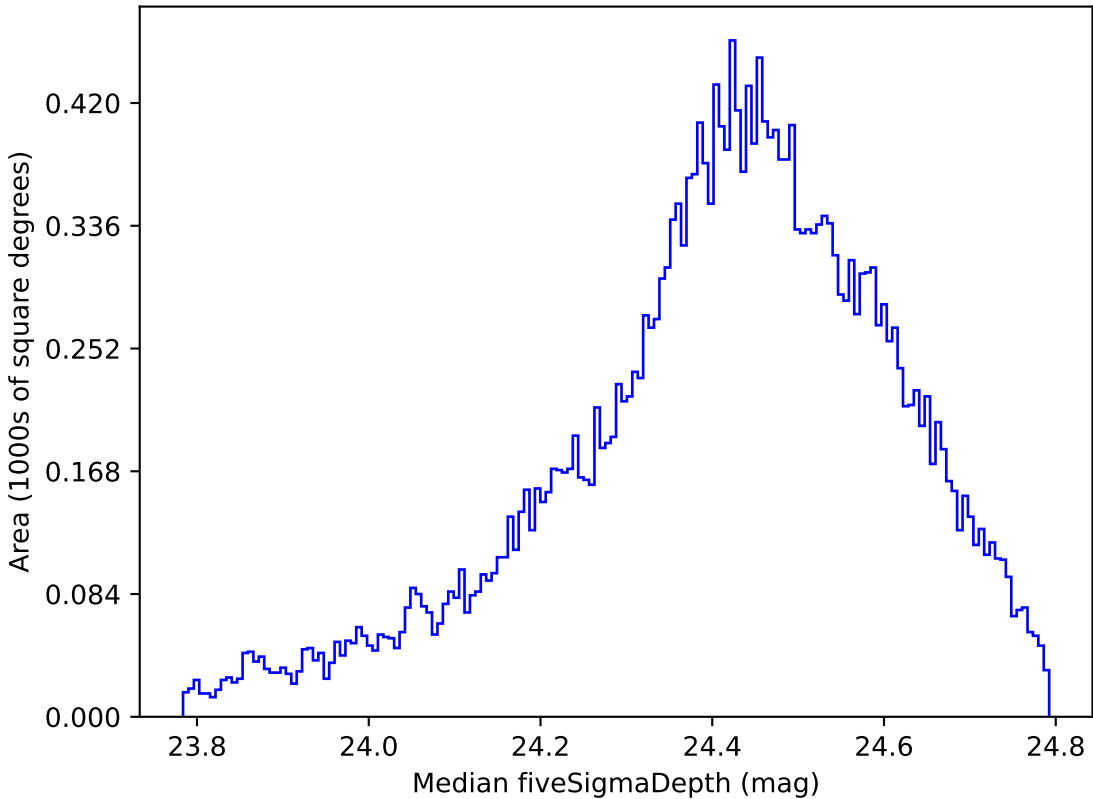
ddf_loaded_fl4_v3.4_10yrs All sky g band: Median fiveSigmaDepth
