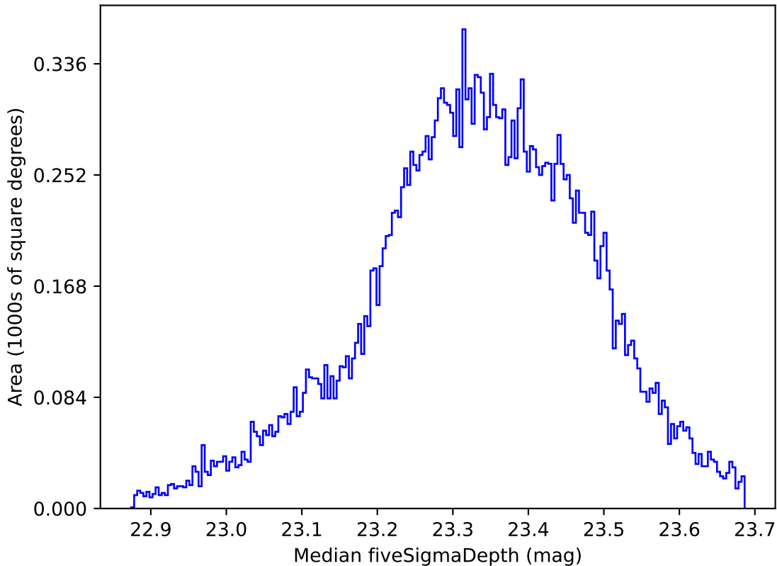
ddf_loaded_fl4_v3.4_10yrs All sky all bands: Median fiveSigmaDepth
