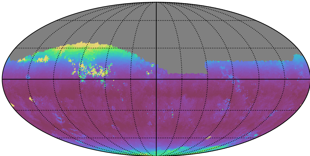
ddf_loaded_fl4_v3.4_10yrs Yr 1 z band: Median airmass
