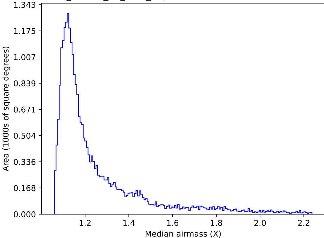
ddf_loaded_fl4_v3.4_10yrs Yr 1 z band: Median airmass
