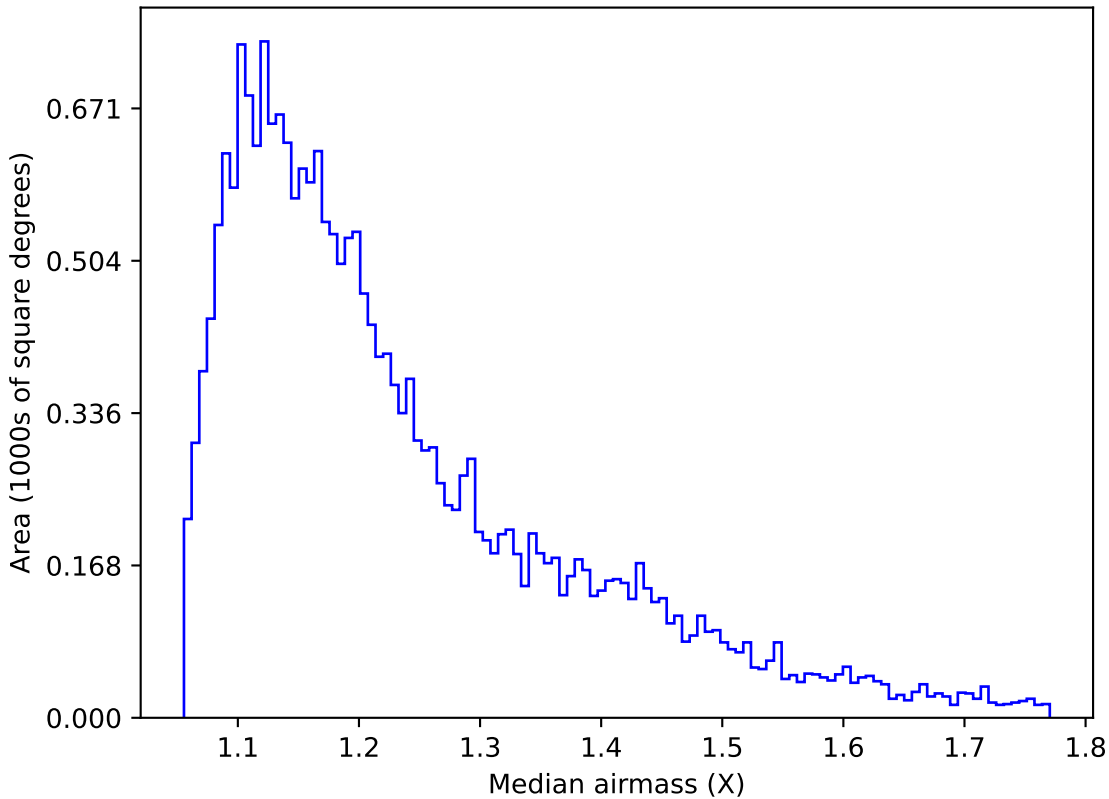
ddf_loaded_fl4_v3.4_10yrs Yr 1 u band: Median airmass
