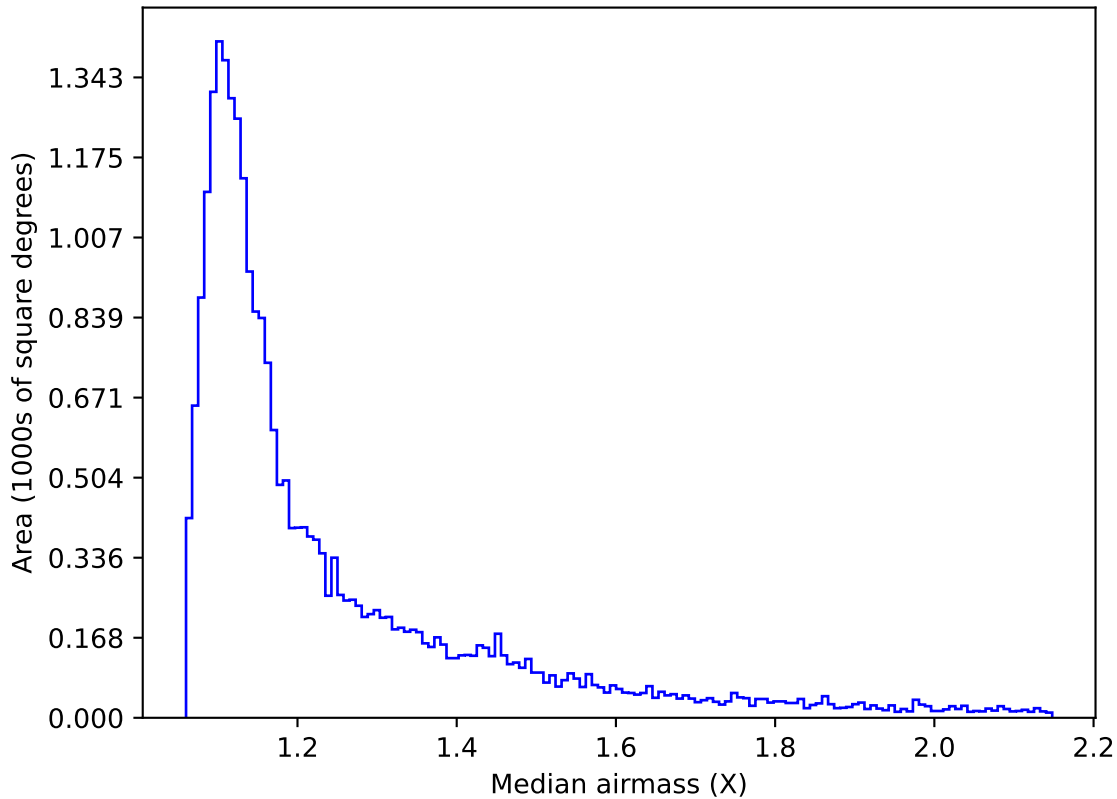
ddf_loaded_fl4_v3.4_10yrs Yr 1 r band: Median airmass
