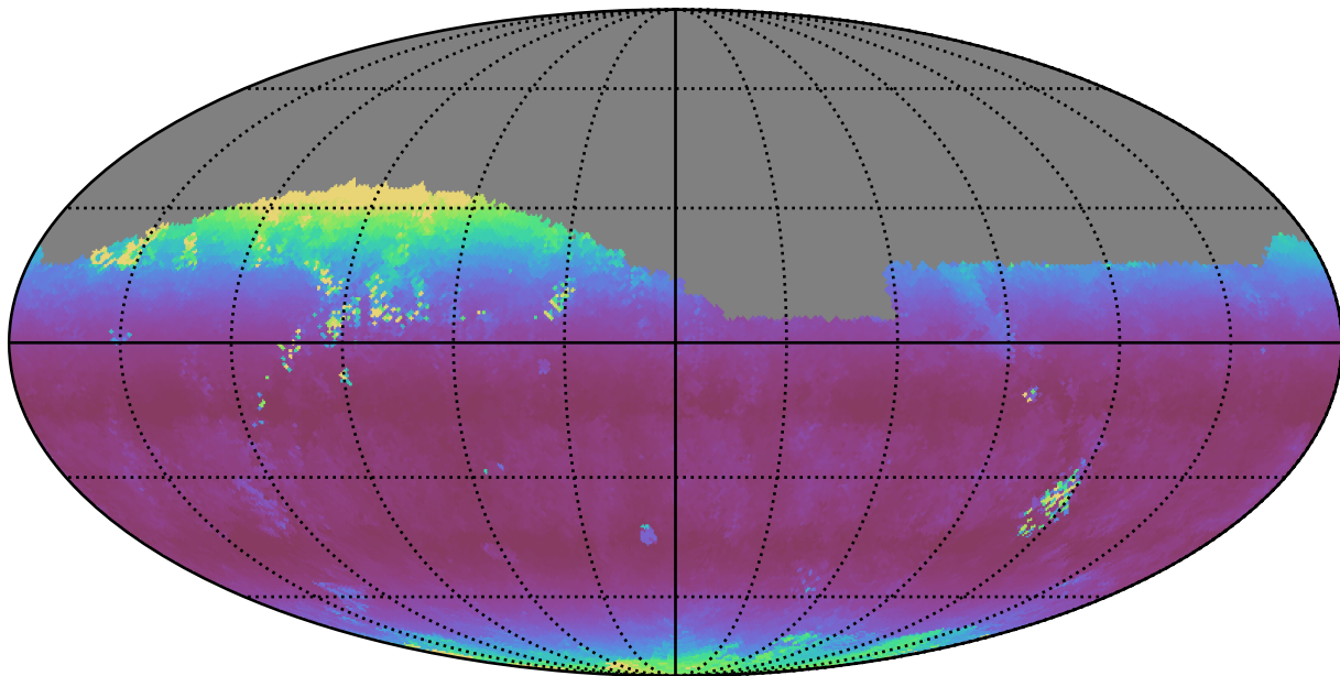
ddf_loaded_fl4_v3.4_10yrs Yr 1 i band: Median airmass
