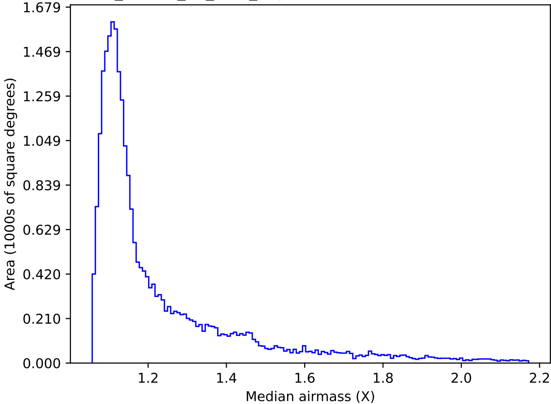
ddf_loaded_fl4_v3.4_10yrs Yr 1 i band: Median airmass
