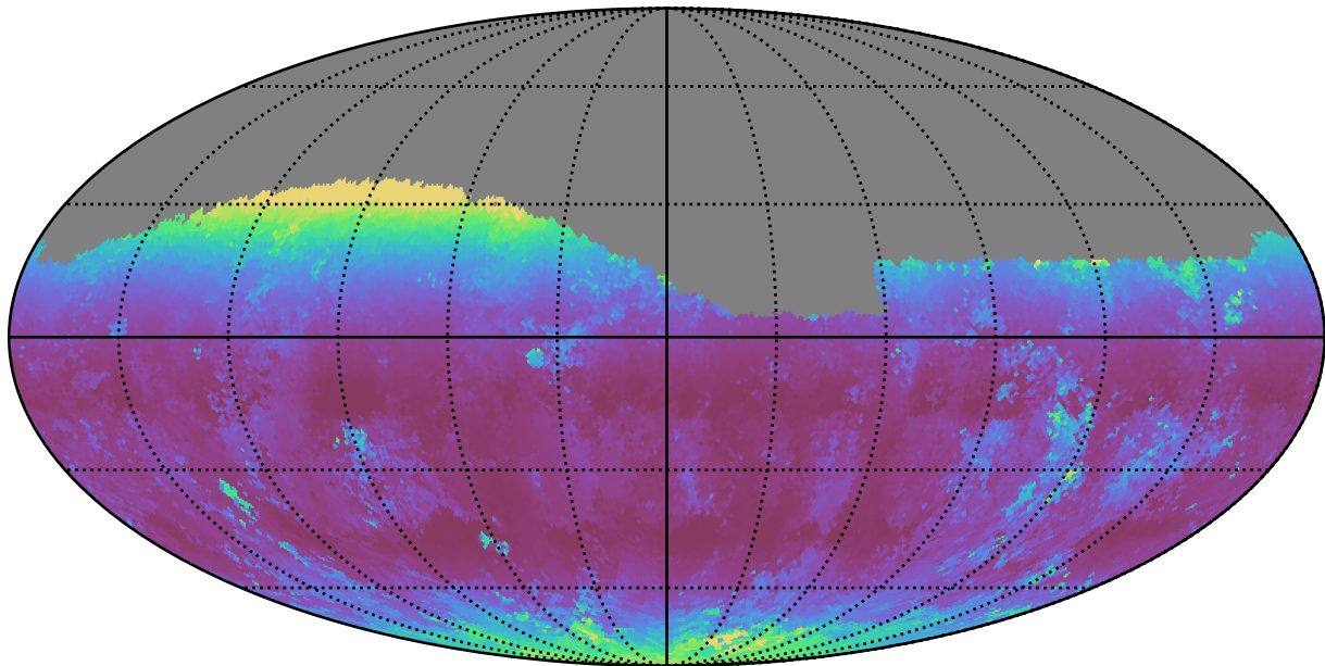
ddf_loaded_fl4_v3.4_10yrs Yr 1 g band: Median airmass
