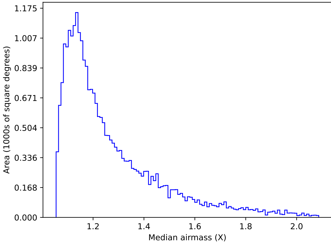
ddf_loaded_fl4_v3.4_10yrs Yr 1 g band: Median airmass
