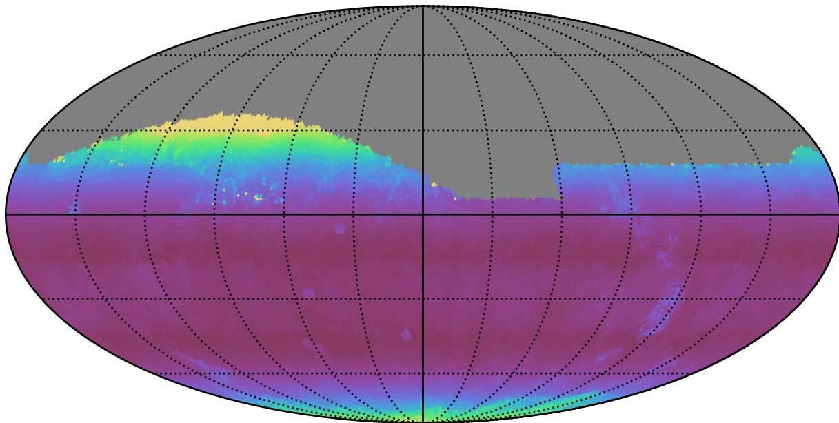
ddf_loaded_fl4_v3.4_10yrs Yr 1 all bands: Median airmass
