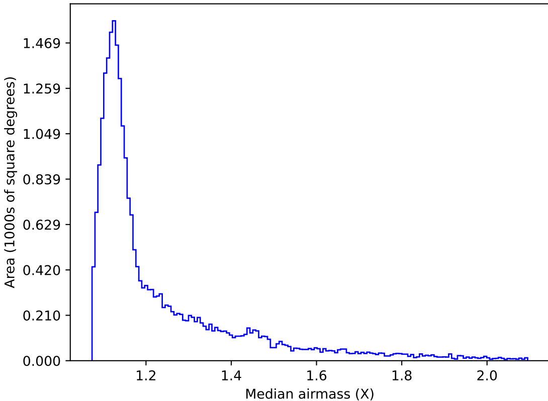
ddf_loaded_fl4_v3.4_10yrs Yr 1 all bands: Median airmass
