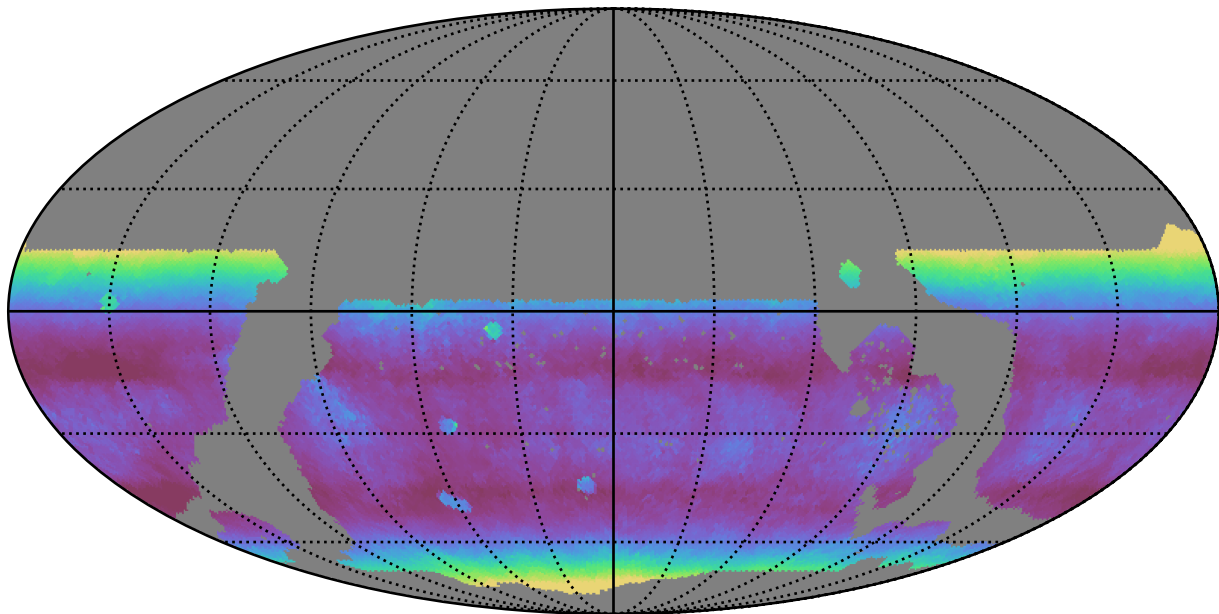
ddf_loaded_fl4_v3.4_10yrs WFD z band: Median airmass
