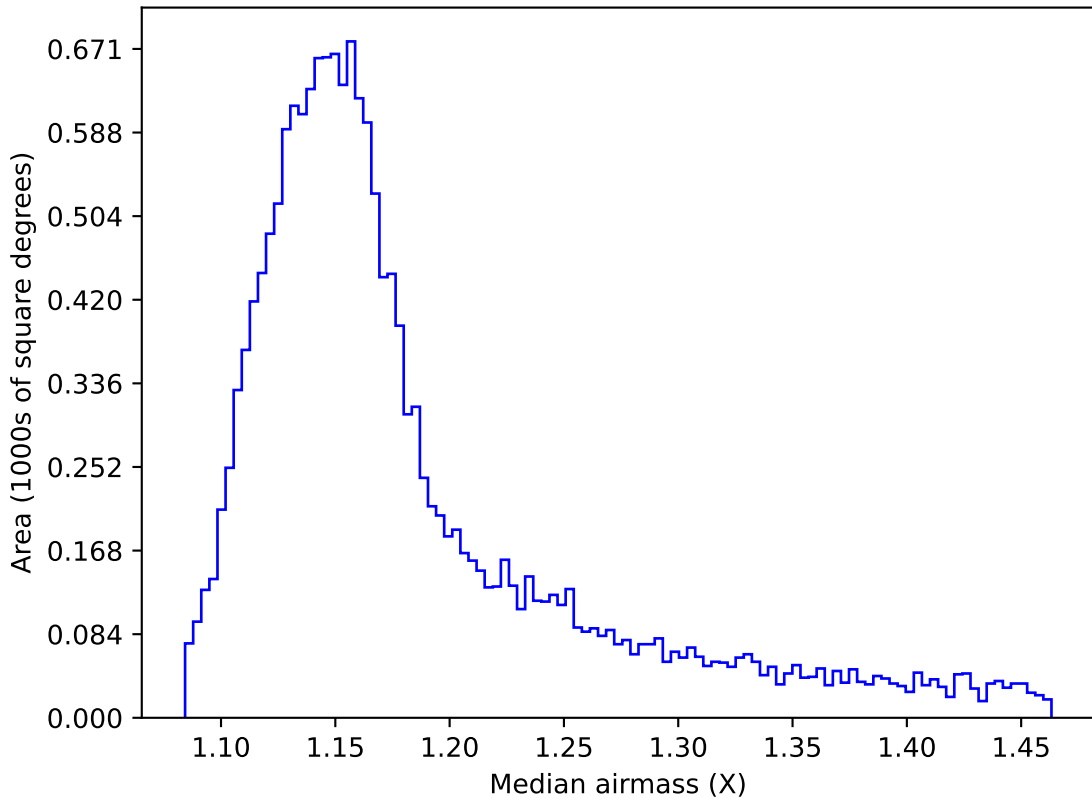
ddf_loaded_fl4_v3.4_10yrs WFD z band: Median airmass
