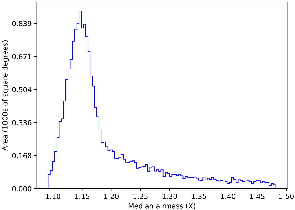
ddf_loaded_fl4_v3.4_10yrs WFD y band: Median airmass
