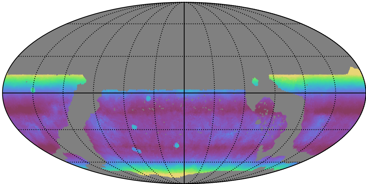
ddf_loaded_fl4_v3.4_10yrs WFD r band: Median airmass
