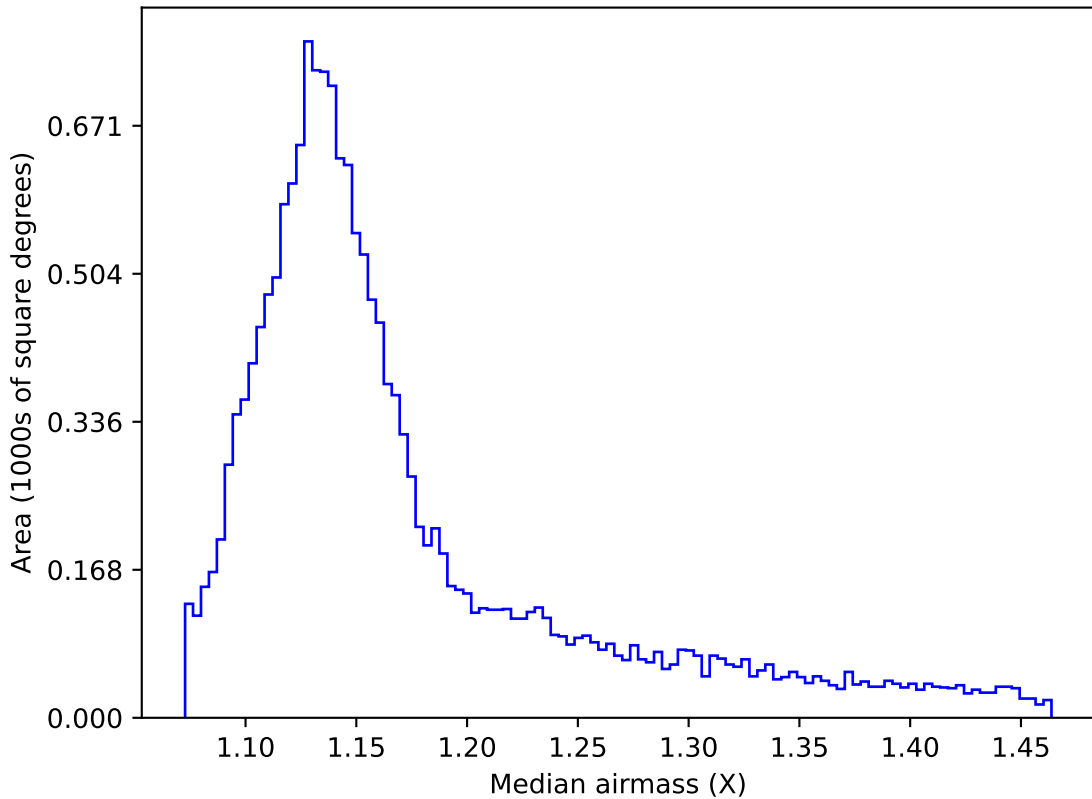
ddf_loaded_fl4_v3.4_10yrs WFD r band: Median airmass
