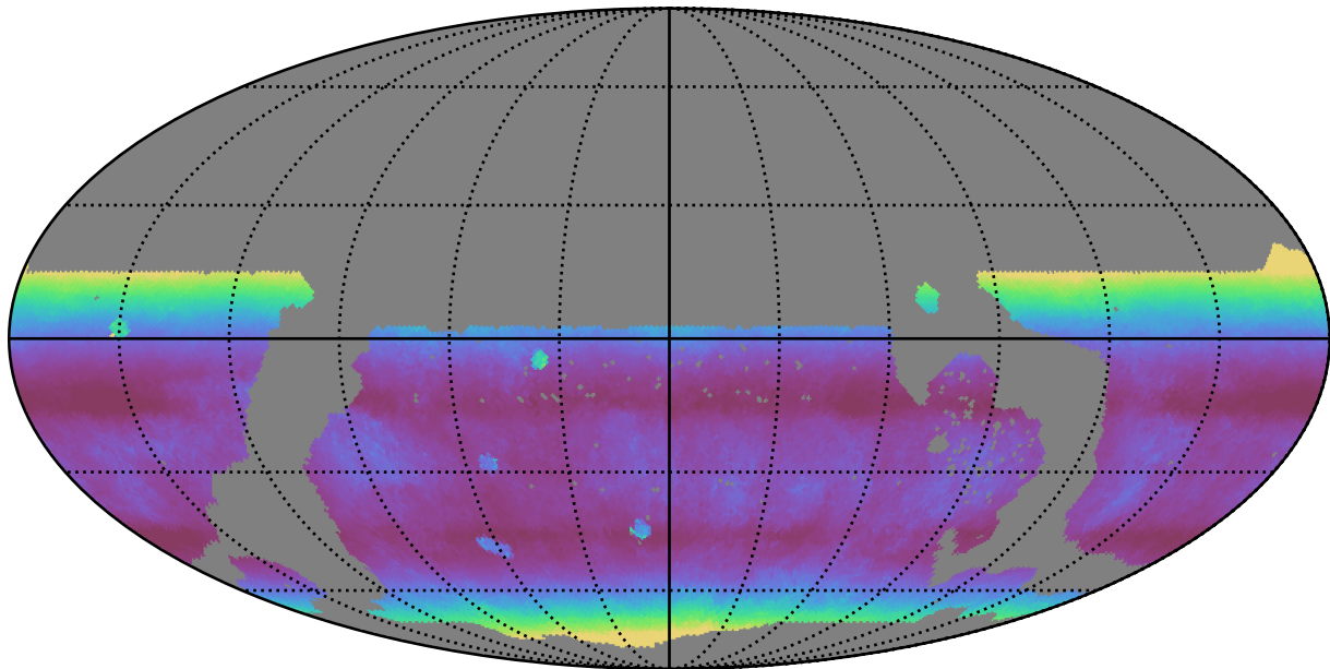
ddf_loaded_fl4_v3.4_10yrs WFD i band: Median airmass
