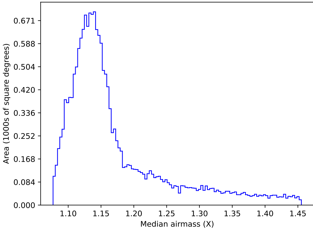
ddf_loaded_fl4_v3.4_10yrs WFD i band: Median airmass
