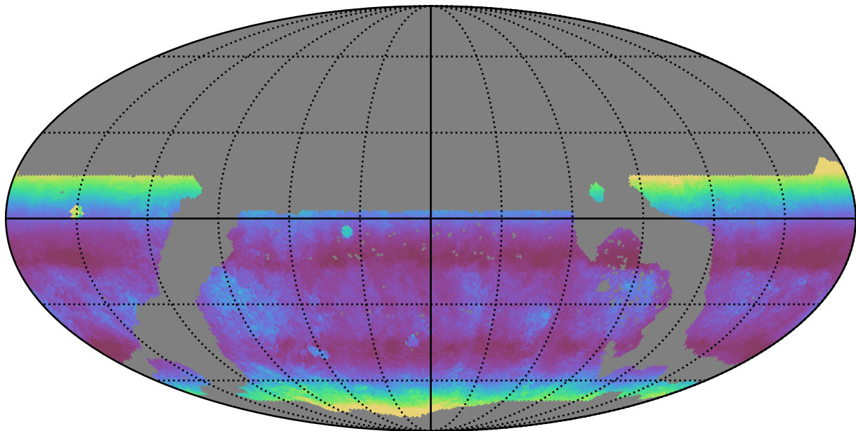
ddf_loaded_fl4_v3.4_10yrs WFD g band: Median airmass
