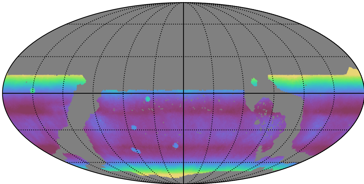
ddf_loaded_fl4_v3.4_10yrs WFD all bands: Median airmass
