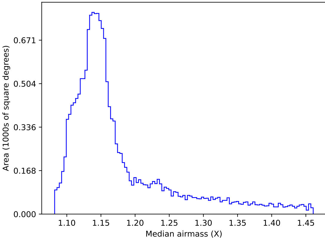
ddf_loaded_fl4_v3.4_10yrs WFD all bands: Median airmass
