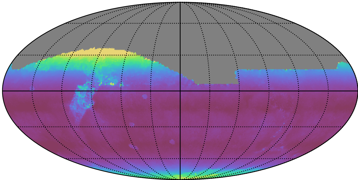
ddf_loaded_fl4_v3.4_10yrs All sky z band: Median airmass
