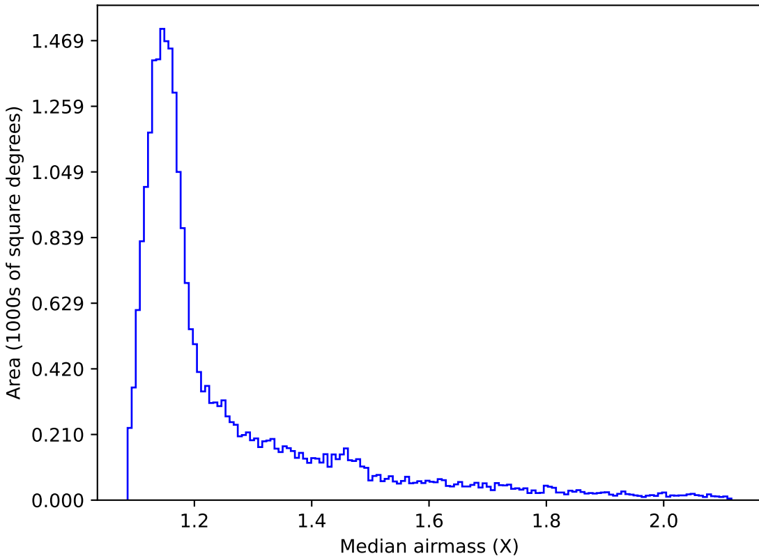
ddf_loaded_fl4_v3.4_10yrs All sky z band: Median airmass
