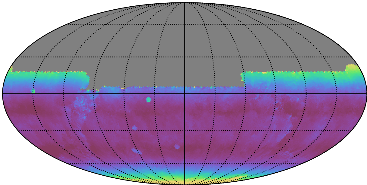
ddf_loaded_fl4_v3.4_10yrs All sky y band: Median airmass
