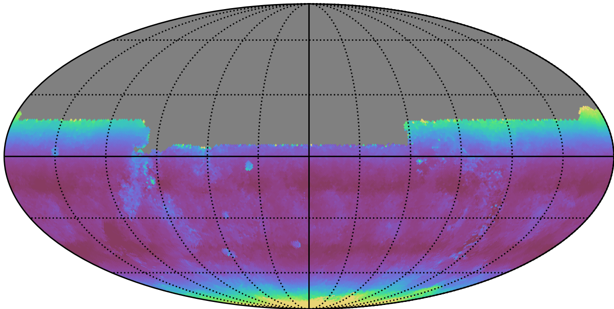
ddf_loaded_fl4_v3.4_10yrs All sky u band: Median airmass
