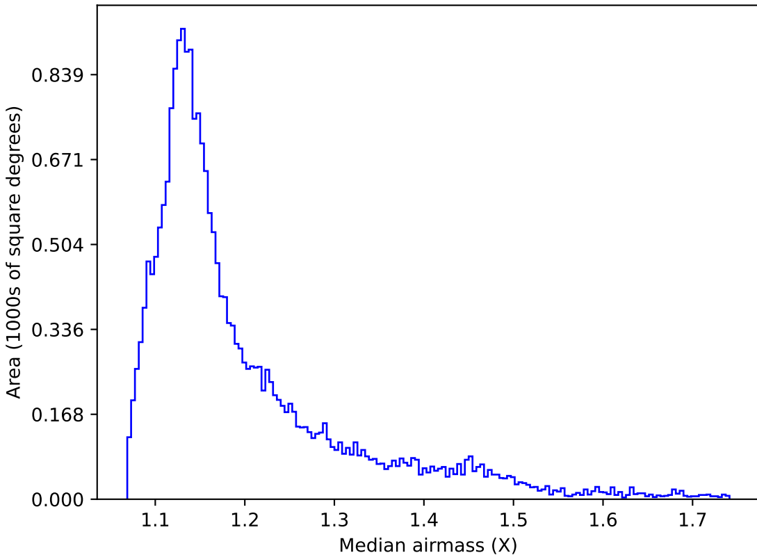
ddf_loaded_fl4_v3.4_10yrs All sky u band: Median airmass
