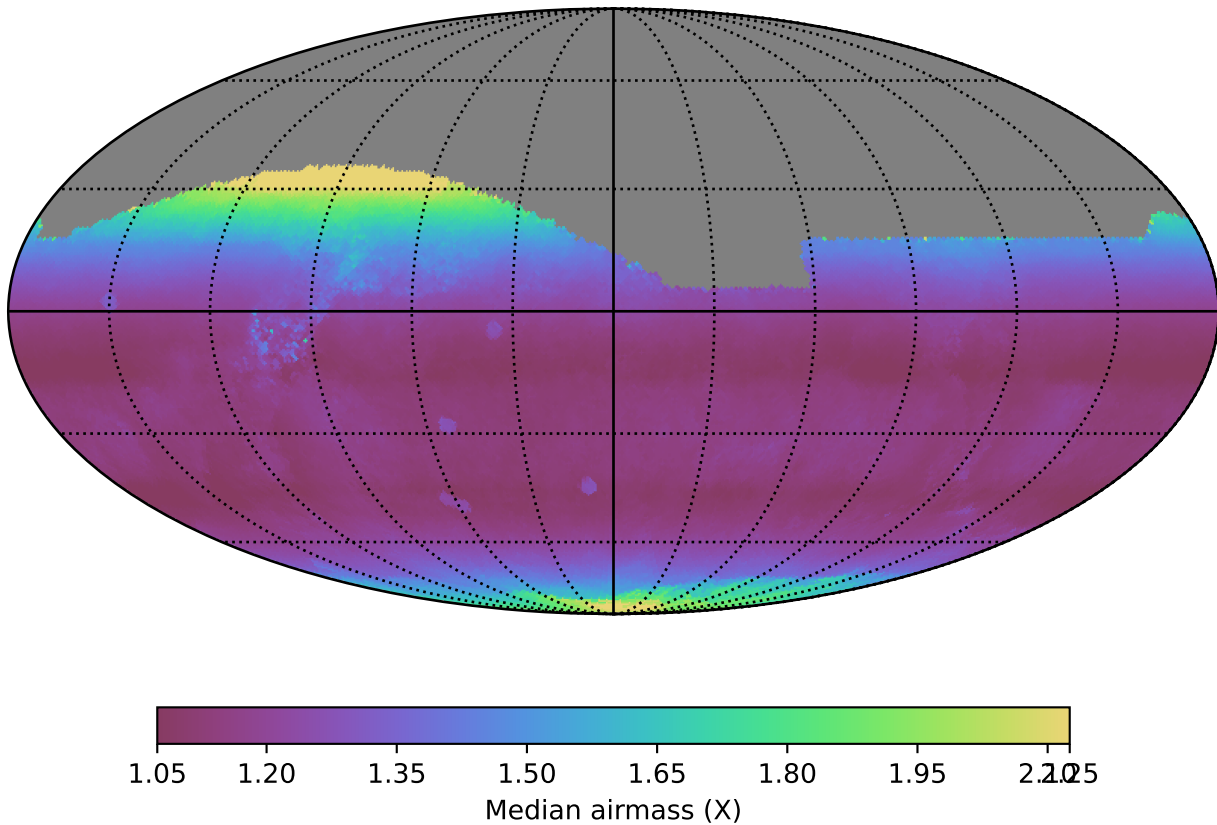
ddf_loaded_fl4_v3.4_10yrs All sky r band: Median airmass
