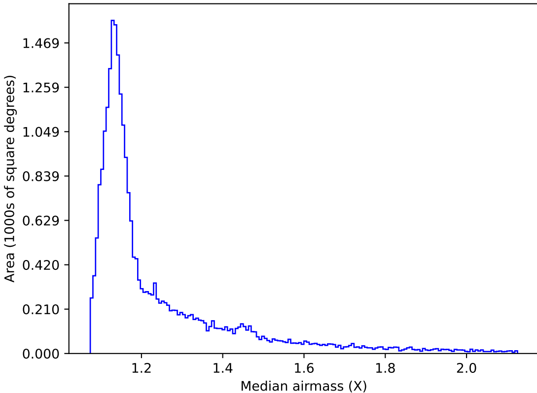
ddf_loaded_fl4_v3.4_10yrs All sky r band: Median airmass
