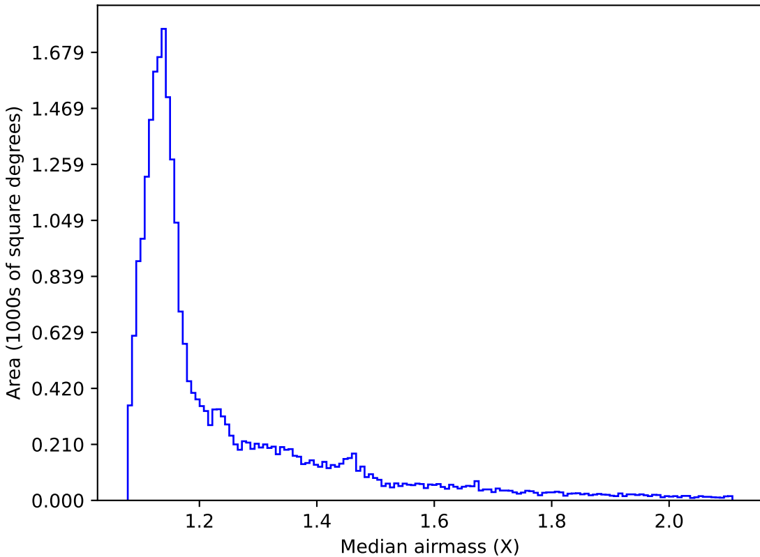
ddf_loaded_fl4_v3.4_10yrs All sky i band: Median airmass
