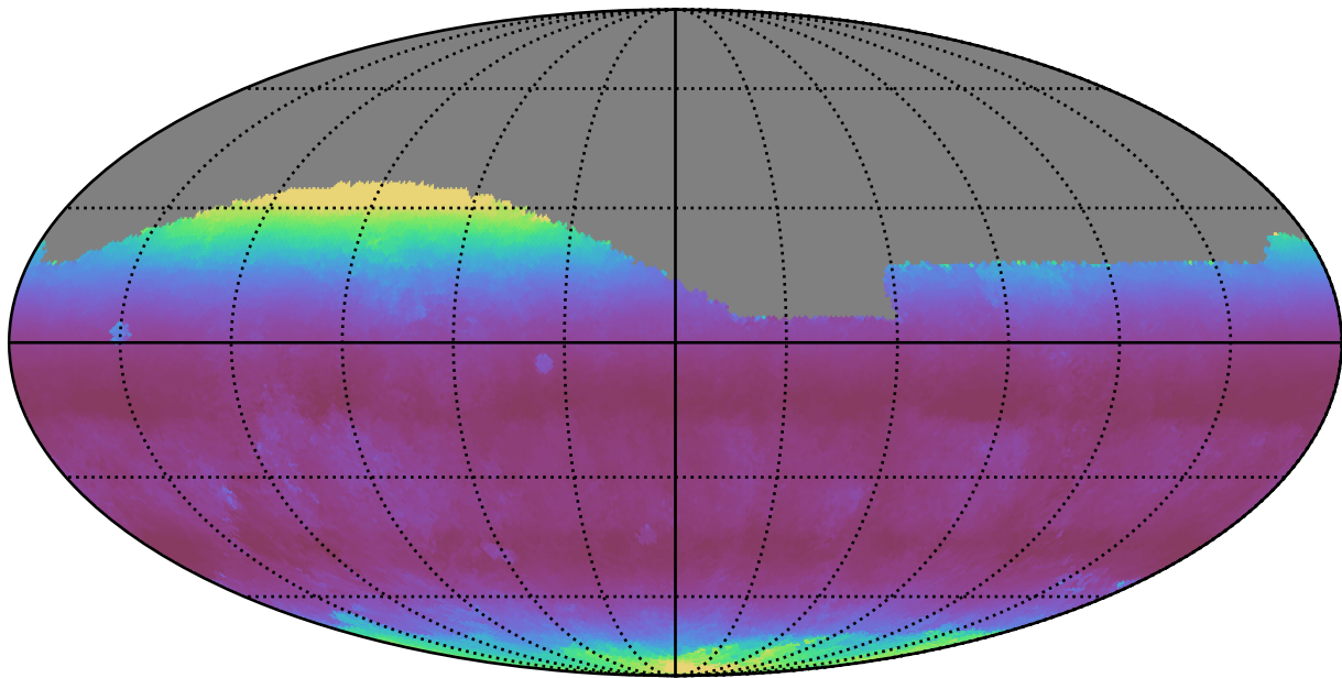
ddf_loaded_fl4_v3.4_10yrs All sky g band: Median airmass
