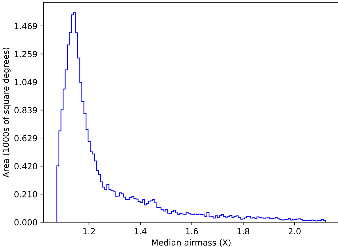
ddf_loaded_fl4_v3.4_10yrs All sky g band: Median airmass
