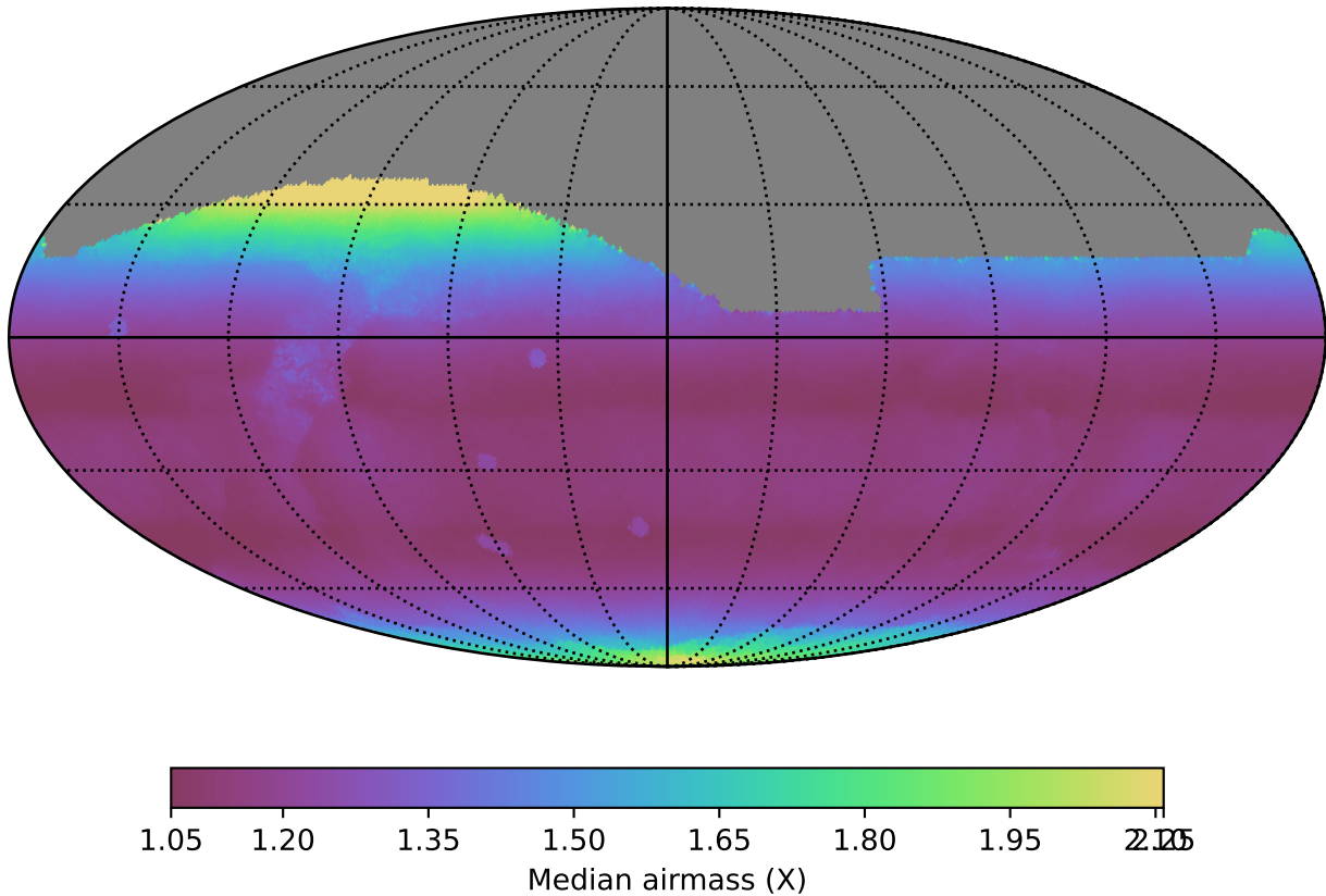
ddf_loaded_fl4_v3.4_10yrs All sky all bands: Median airmass
