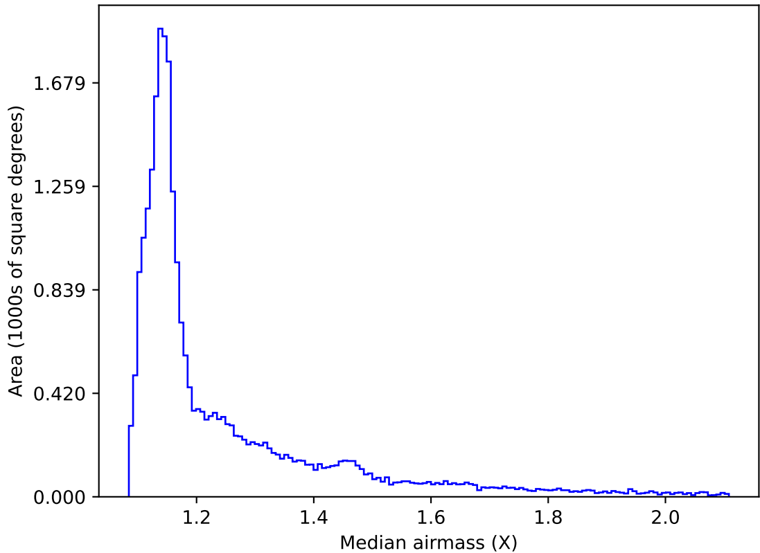
ddf_loaded_fl4_v3.4_10yrs All sky all bands: Median airmass
