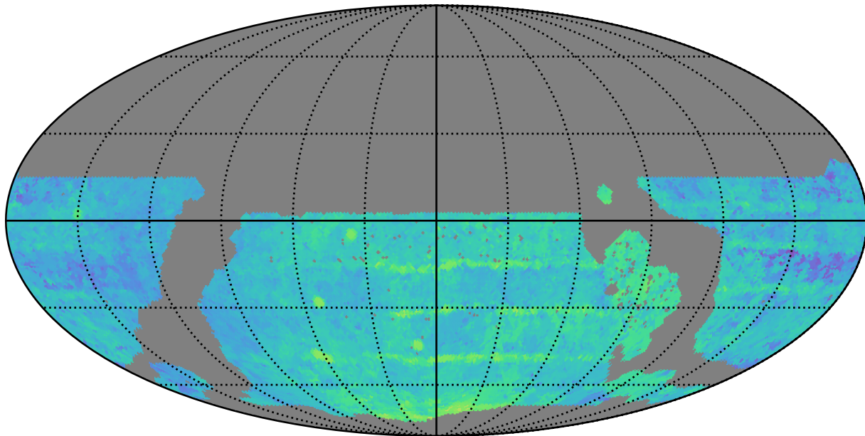
ddf_loaded_fl4_v3.4_10yrs WFD z band: Median Season Length
