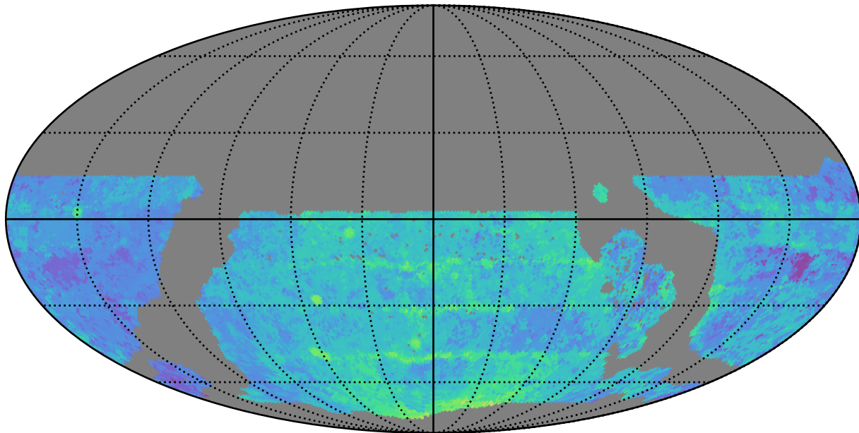
ddf_loaded_fl4_v3.4_10yrs WFD y band: Median Season Length
