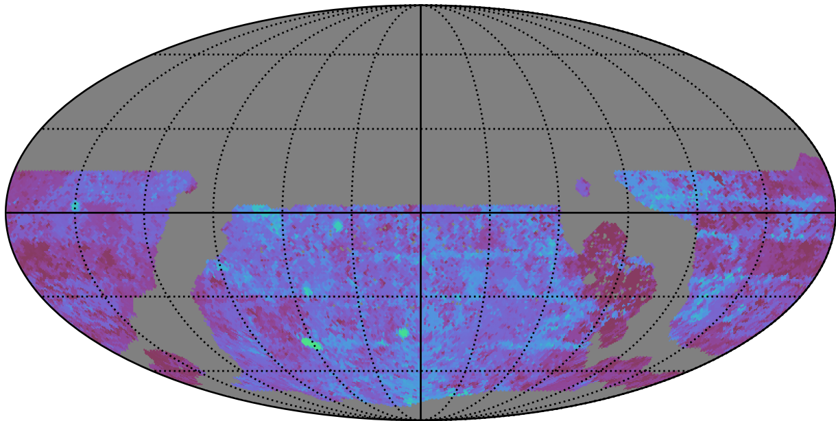
ddf_loaded_fl4_v3.4_10yrs WFD u band: Median Season Length
