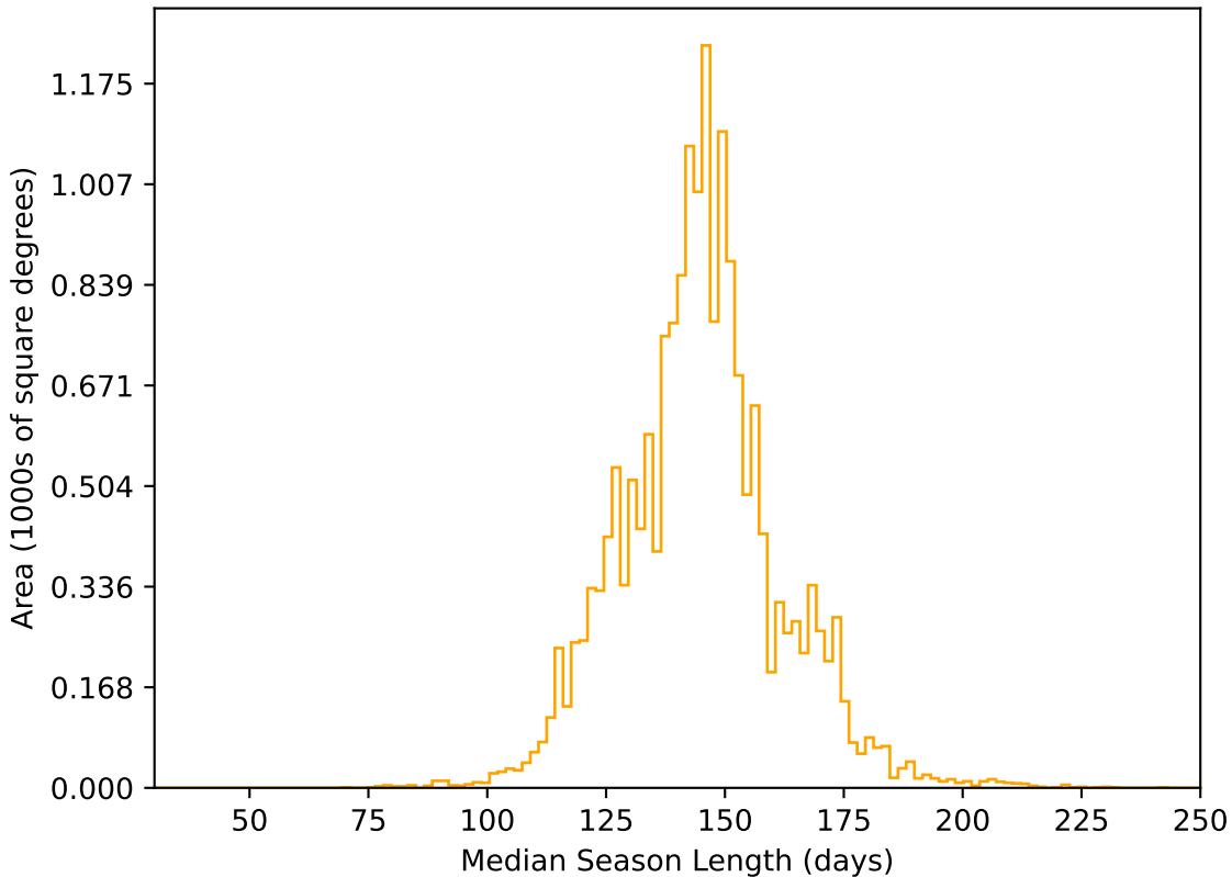
ddf_loaded_fl4_v3.4_10yrs WFD r band: Median Season Length
