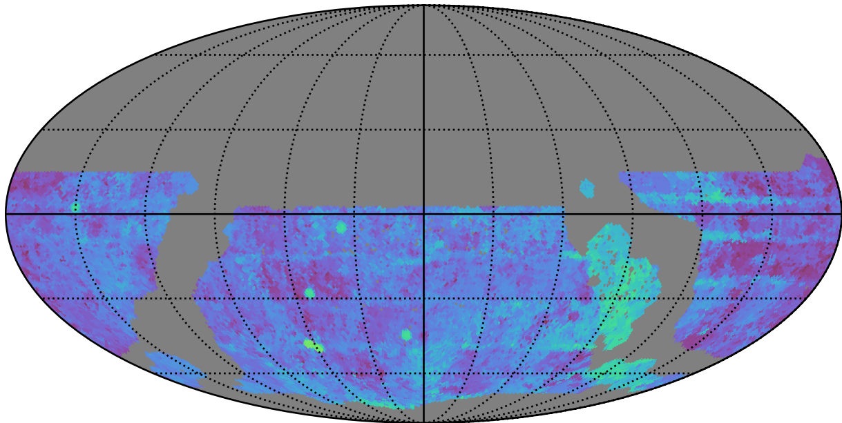
ddf_loaded_fl4_v3.4_10yrs WFD g band: Median Season Length
