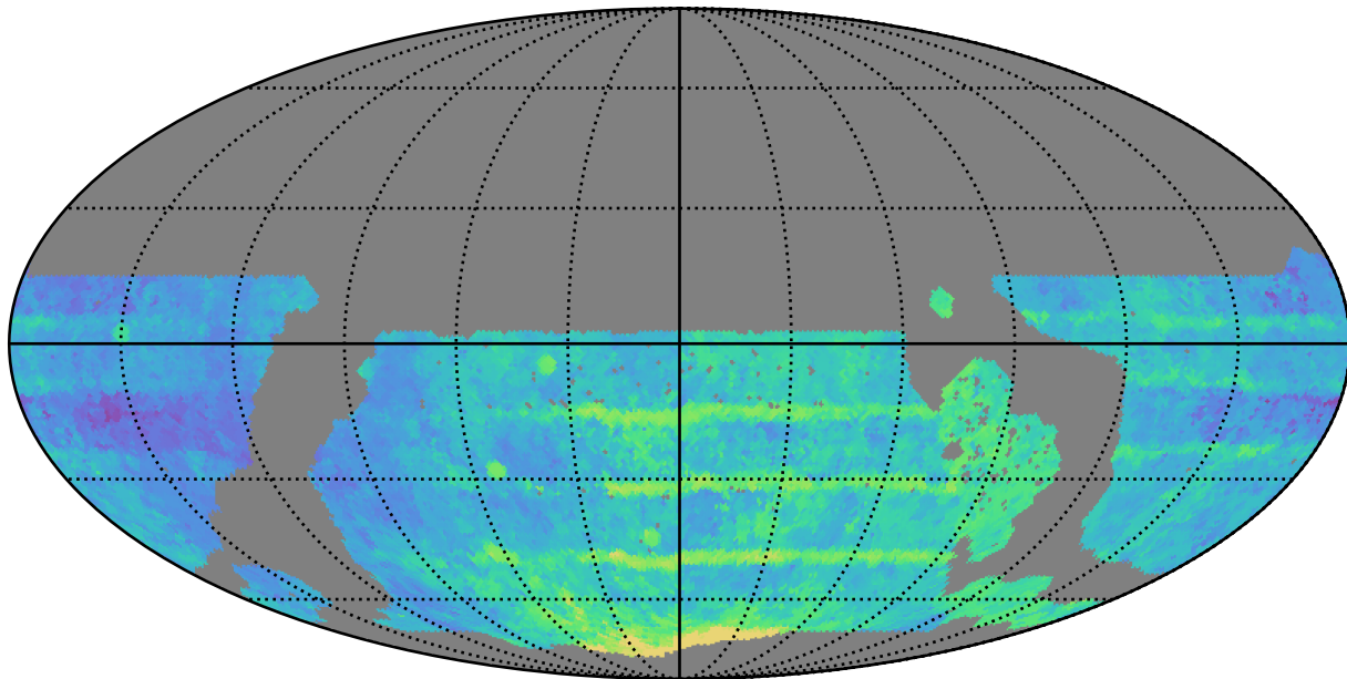
ddf_loaded_fl4_v3.4_10yrs WFD all bands: Median Season Length
