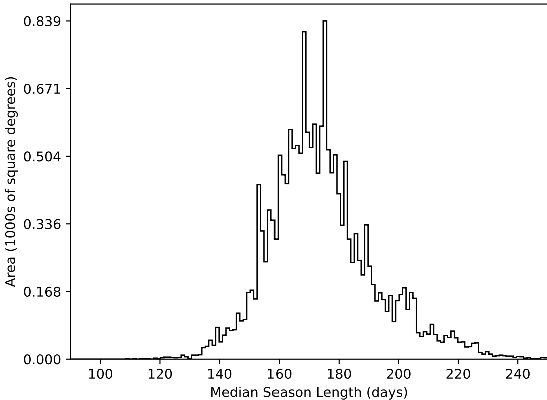
ddf_loaded_fl4_v3.4_10yrs WFD all bands: Median Season Length
