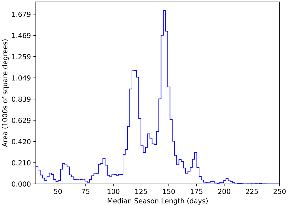
ddf_loaded_fl4_v3.4_10yrs All sky y band: Median Season Length
