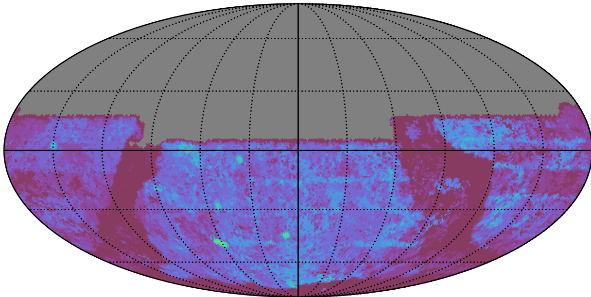
ddf_loaded_fl4_v3.4_10yrs All sky u band: Median Season Length
