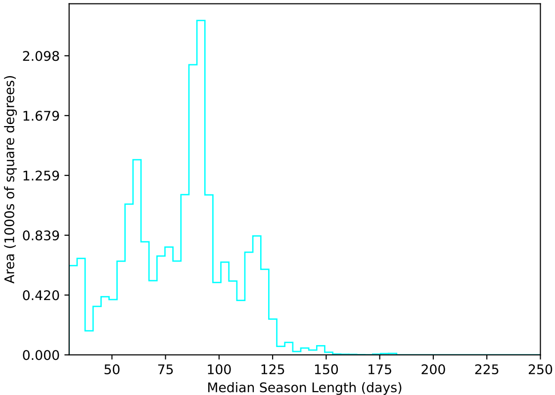
ddf_loaded_fl4_v3.4_10yrs All sky u band: Median Season Length
