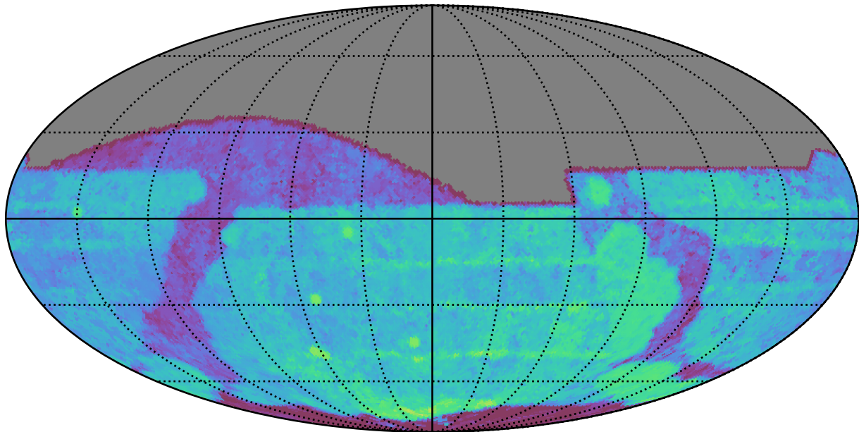
ddf_loaded_fl4_v3.4_10yrs All sky r band: Median Season Length
