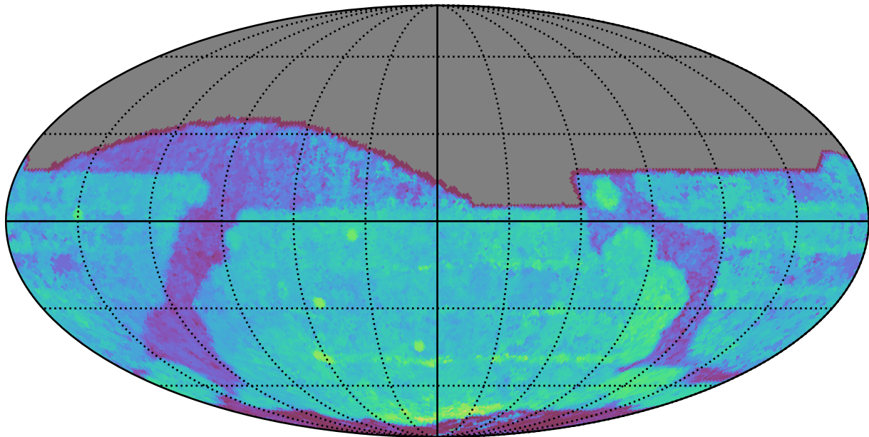
ddf_loaded_fl4_v3.4_10yrs All sky i band: Median Season Length
